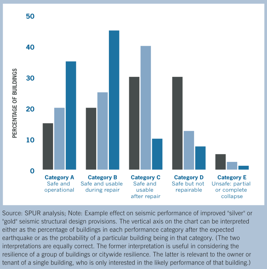
FIGURE A: HOW WOULD "SEISMIC GOLD" AND "SEISMIC SILVER" BUILDINGS FARE AFTER AN EARTHQUAKE?
